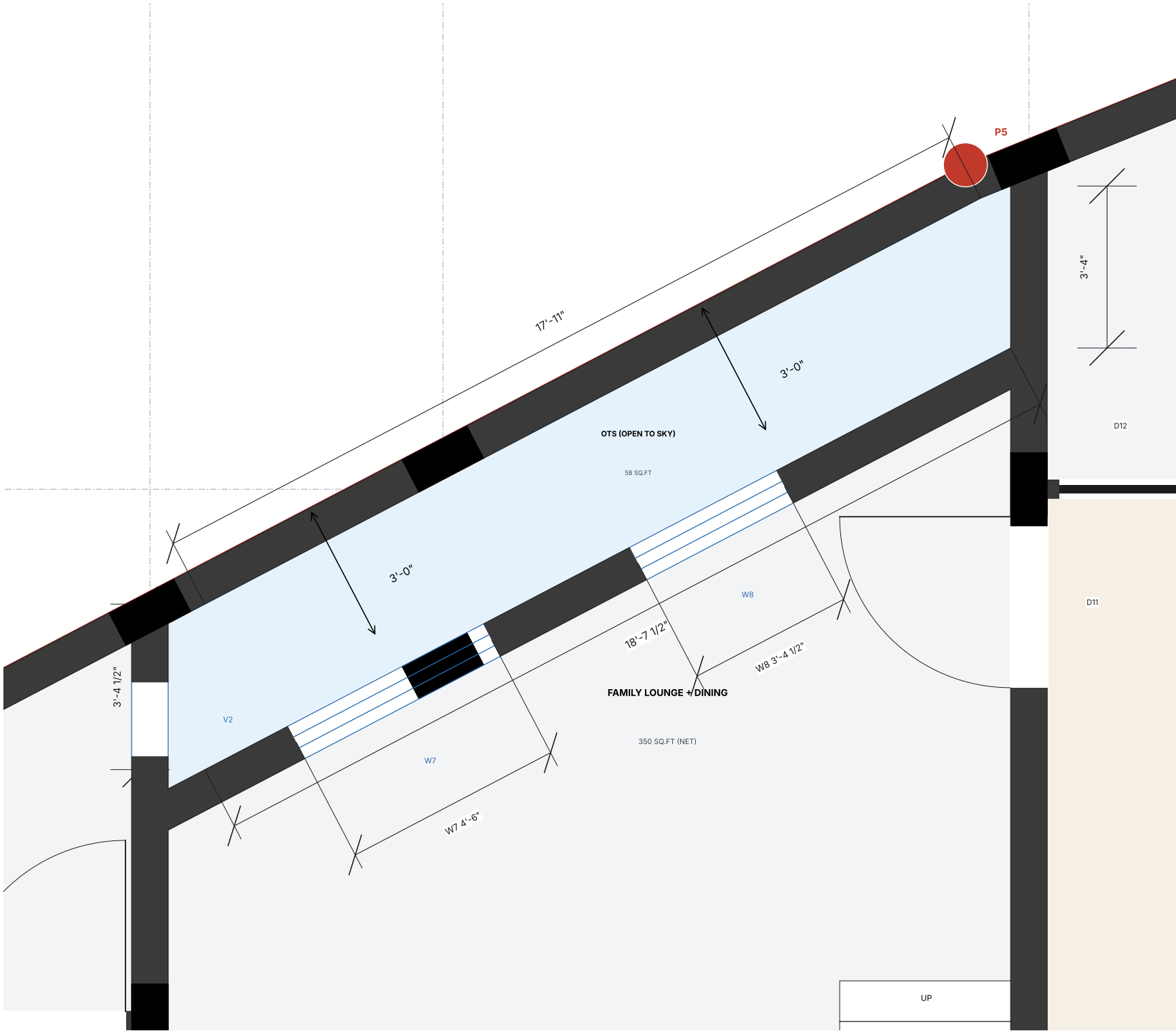
ENLARGED PLAN : OTS (3/8"=1'-0")
