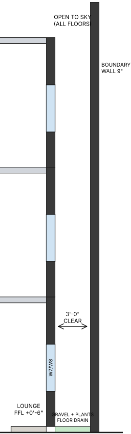
SECTION C-C : OTS (LIGHT WELL)
